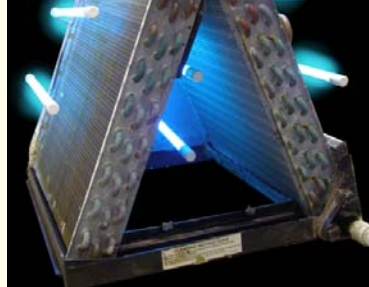
UV light AC coil requires 6 lamps
